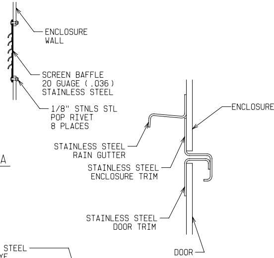
SECTION Z-Z
