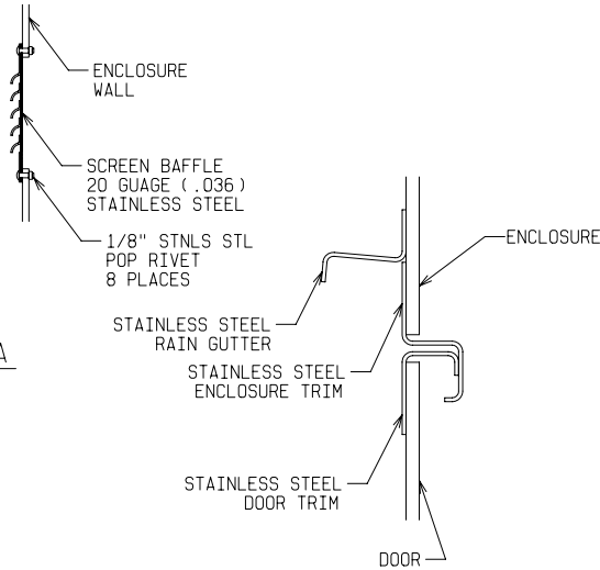
SECTION Z-Z
