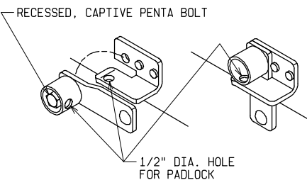
LATCH DETAIL
