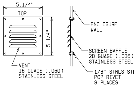
LOUVER DETAIL
